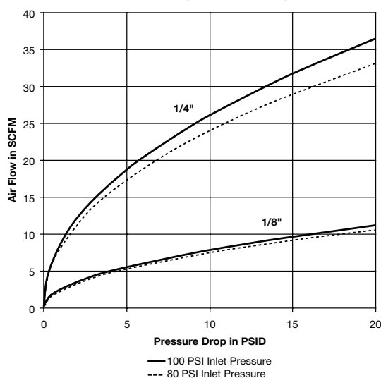
Performance HF Series (1/8" & 1/4" sizes)
