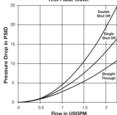
Spectrum Series (1/8") Test Fluid: Water
